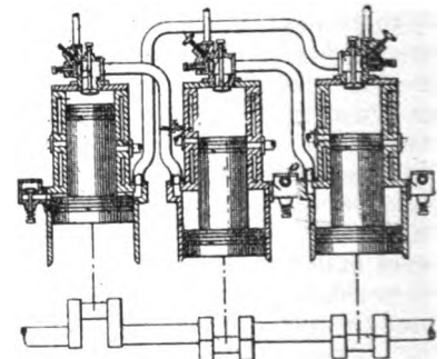
Differential Piston Two-Cycle Engine
